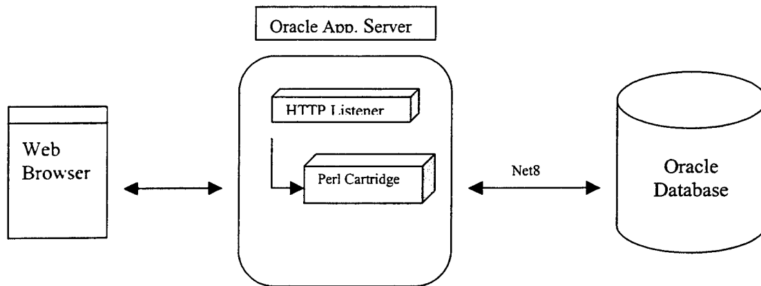
Figure 4.7 Perl Cartridge in OAS
